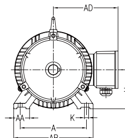
B3 mounting construction
