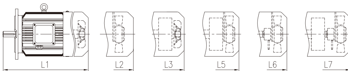
MP motor length and weight
