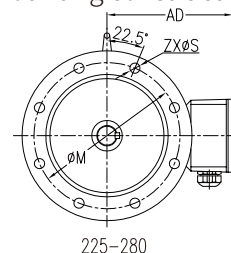
B5 mounting construction
