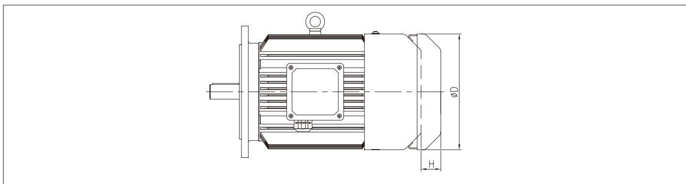
◆ Dimensions of rainproof cover
