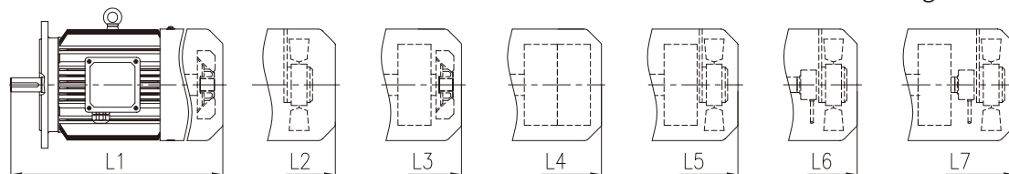
MU motor length and weight
